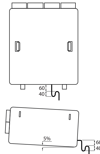
PIC 05: Condensate siphon in the KCX AHU and declination of the suspended AHU version.
