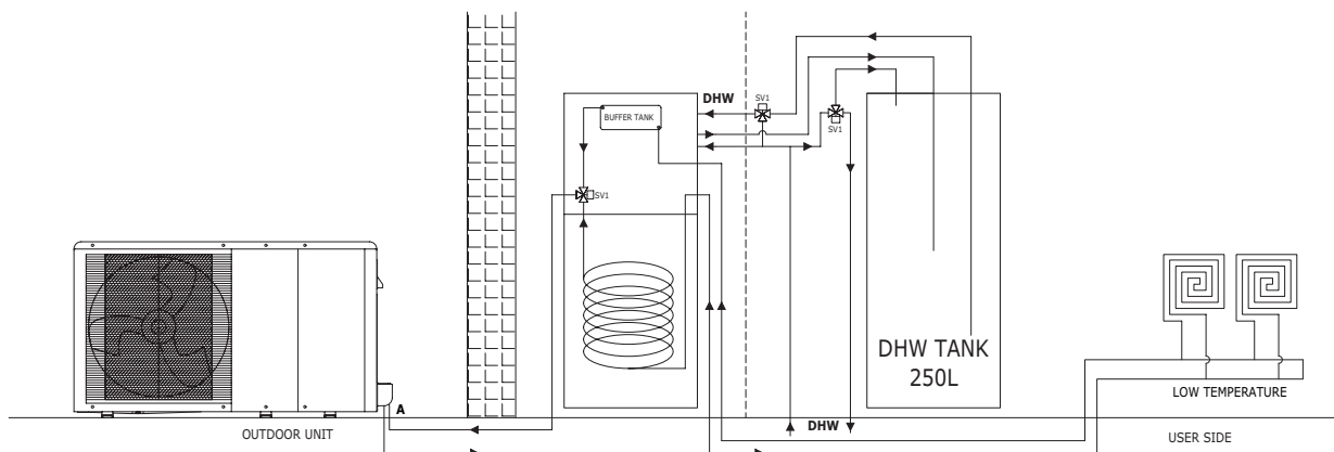
250L DHW tank
